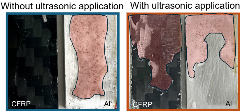
Fig. 5 Fracture surface with and without ultrasonic application at 298K
