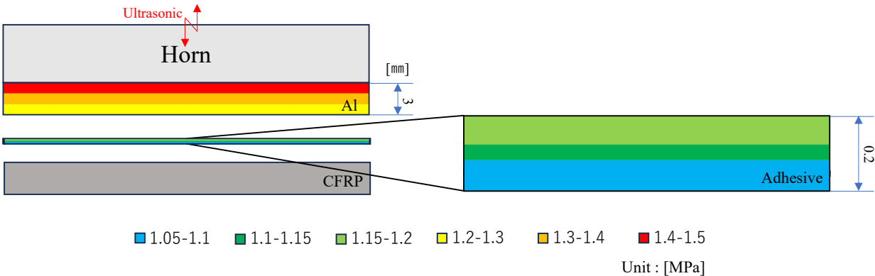
Fig. 3 Sound pressure distribution simulation from the Al side Table. 1 Adhesive bond strength at 298K with and without ultrasonic application Ultrasonic Application Adhesive Bond strength, \tau [MPa] Average Bond strength, \tau Ave. [MPa] ○ 14.57 11.75 11.42 12.58 - 8.92 8.67 6.98 8.19
